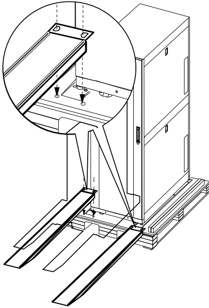
PDU Cabinet
